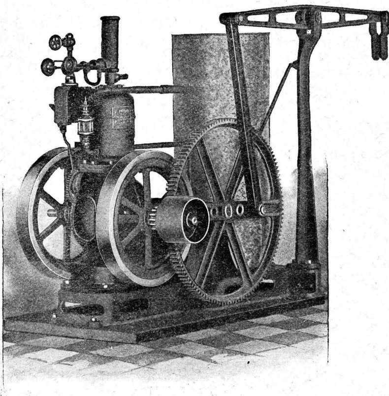
VERTICAL ENGINE AND PUMP JACK
