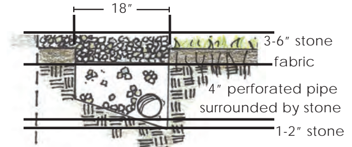
Figure 2. Profile for slowly draining soils.
