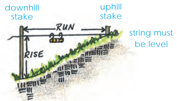
Figure 1. Determine the slope of the landscape before digging.
