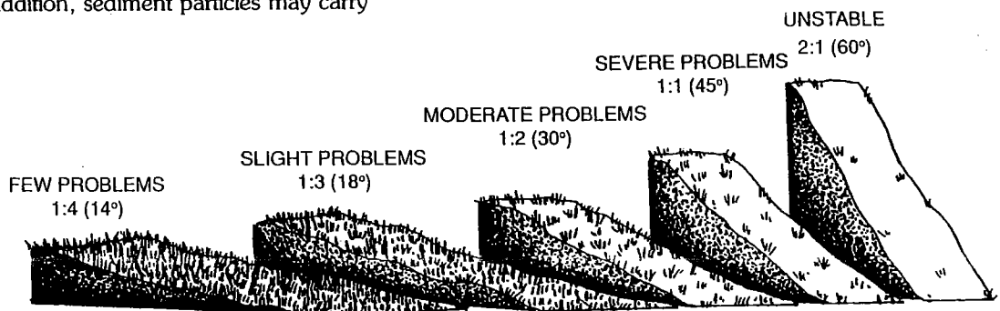
COMPARISON OF SLOPE ANGLES AND STABILITY
