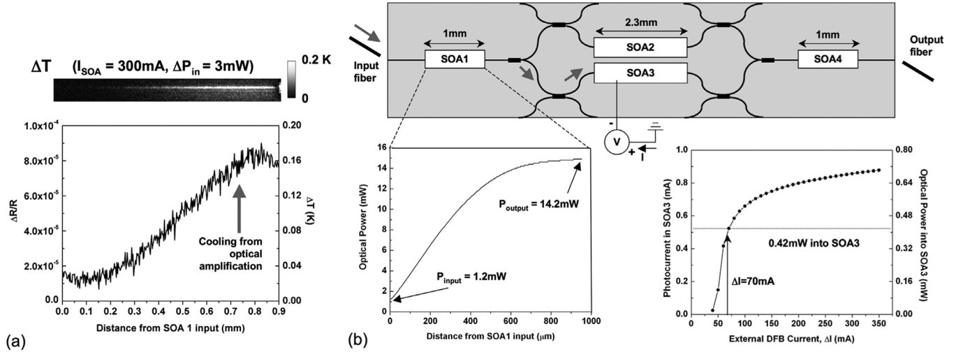
Fig. 4. (a) Thermal image (top) and temperature profile along SOA ridge for cooling from optical amplification when the SOA is biased at 300 mA (b) (top) Schematic of a part of an Aliphion PIC used in the measurements. SOA1 and SOA4 are 1 mm and SOA2 and SOA3 are 2.3 mm in length. SOA1 and SOA4 are fiber coupled. (bottom left) Optical power in SOA1 calculated from the thermal image, for \Delta P_{\text{inj}} = 3 mW into the input fiber, a fiber coupling loss of 4 dB, and an SOA1 bias current of 300 mA. (bottom right) Photocurrent measured in SOA3 as a function of external DFB laser bias current, for SOA1 biased at 300 mA and SOA3 biased at -2 V. The conversion factor of 0.8 mW/mA is used for the photocurrent measurements, assuming one electron-hole pair is generated per photon absorbed. The vertical arrow shows the DFB laser bias point used for the measurement.
