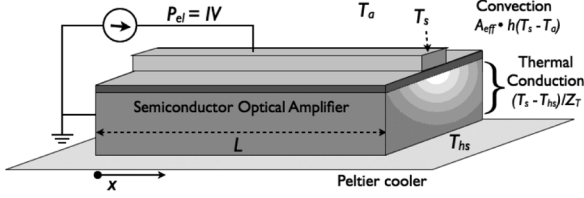
Fig. 1. Schematic of an SOA under normal operating conditions, where P_{el} represents electrical power injected into the device, Z_T represents the thermal impedance from the active region to the substrate, and A_{eff} \cdot h represents convective cooling from the surface.
