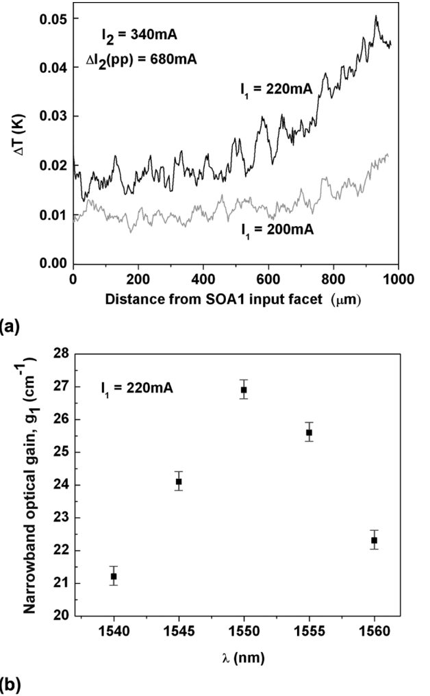
Fig. 6. (a) Temperature profile along the ridge of SOA1 in Fig. 4, biased at 200 mA and 220 mA, using modulated ASE of SOA2 as the light source. A cooling of about 30 mK is observed at the output facet at 220 mA. A broadband material gain of about 21 \text{ cm}^{-1} is obtained from this profile at 220 mA. (b) Measured narrowband material gain of SOA1 at 220 mA, at different wavelengths of the injected light. The spectrally averaged gain from this plot is 24 \text{ cm}^{-1} which is close to the broadband gain.
