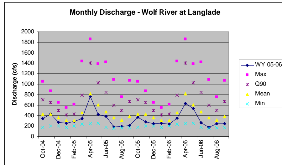
Figure 10. Monthly discharge during water year 2005-6 compared to gauge statistics for select Fox-Wolf streams
