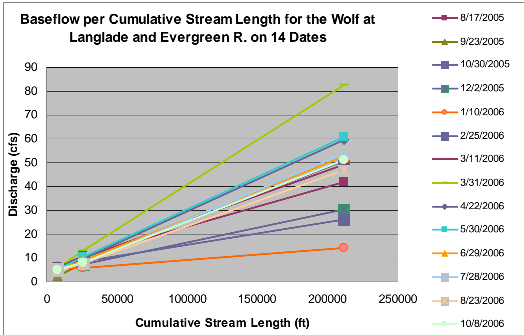
Figure 16. Baseflow per cumulative stream length for the Wolf at Langlade and Evergreen Rivers watershed on 14 dates. Note the small degree of variability at small cumulative stream lengths.
