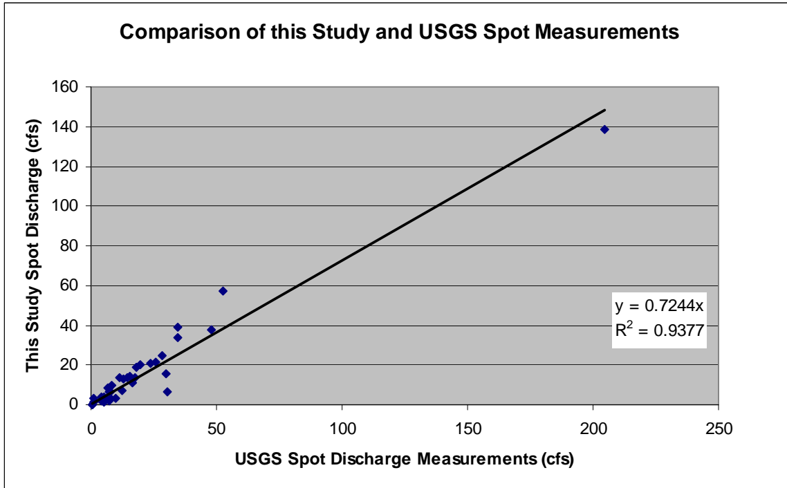
Figure 15. Comparison of this study and USGS spot discharges.
