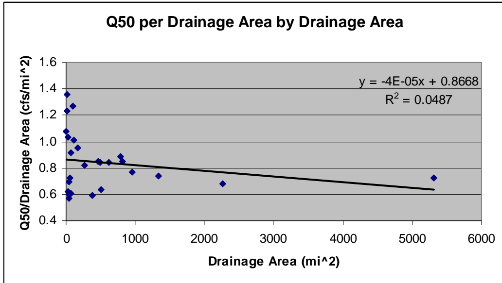
Figure 11. Q_{50} per drainage area at USGS daily gauge stations
