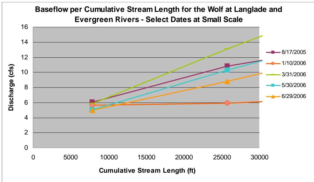
Figure 17. Baseflow per cumulative stream length at small scale.
