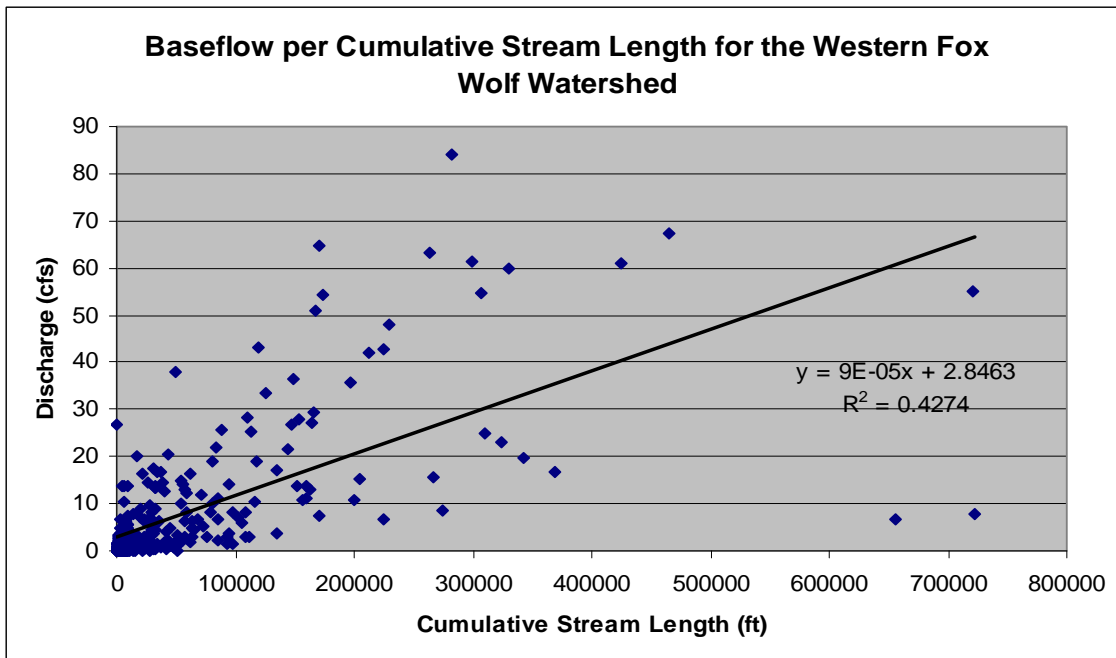
Figure 13. Baseflow discharge compared with cumulative stream length. Note the correlation is poor ( R^2 < 0.5 ) when all data points are considered simultaneously.
