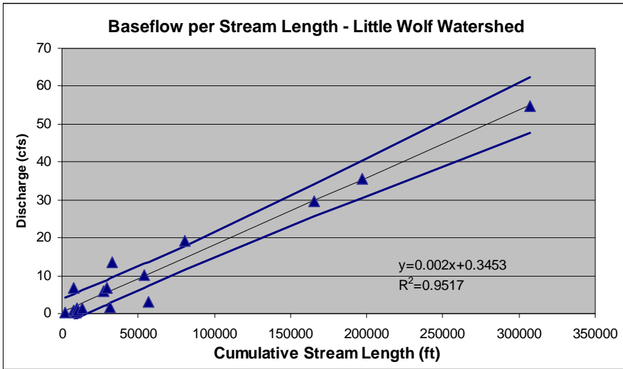
Figure 14. Baseflows per cumulative stream length in 11 subwatersheds of the western Fox-Wolf basins.
