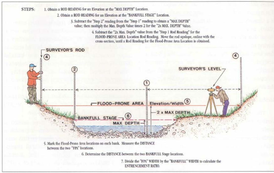
Figure 4. Determining Entrenchment Ratio
