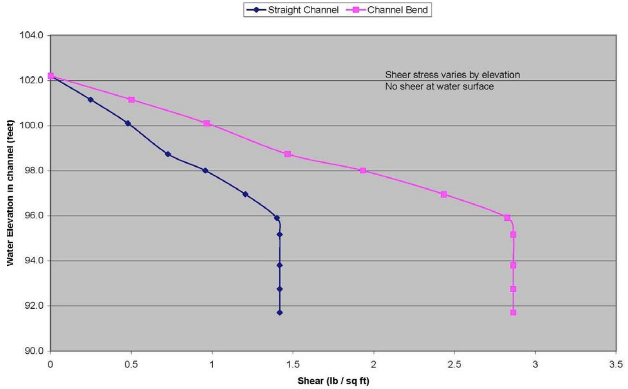
Calculated Shear Stress on Stream Bank
