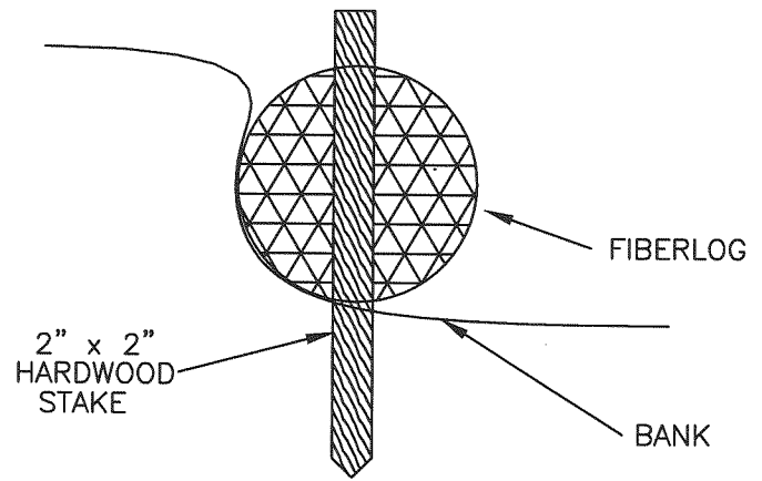
2" x 2" HARDWOOD STAKE
