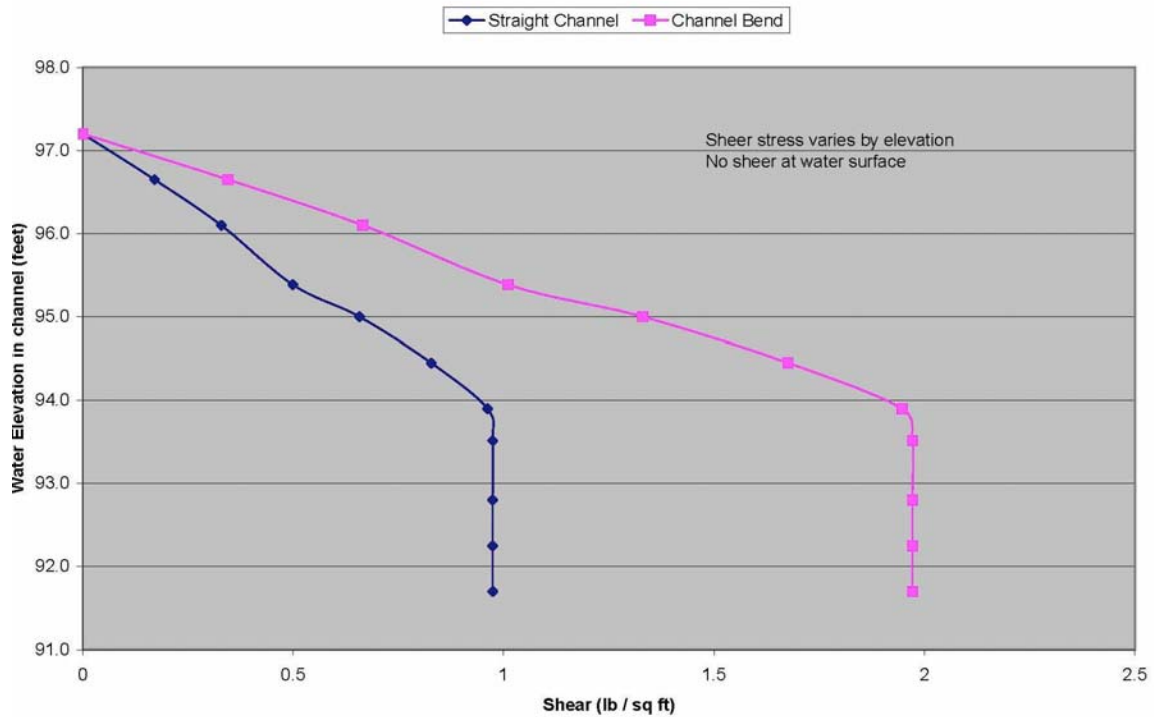
Calculated Shear Stress on Stream Bank
