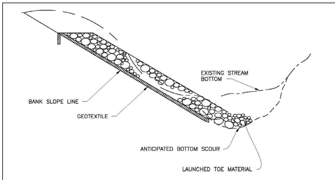
Figure WI-16-8b (after launching)
