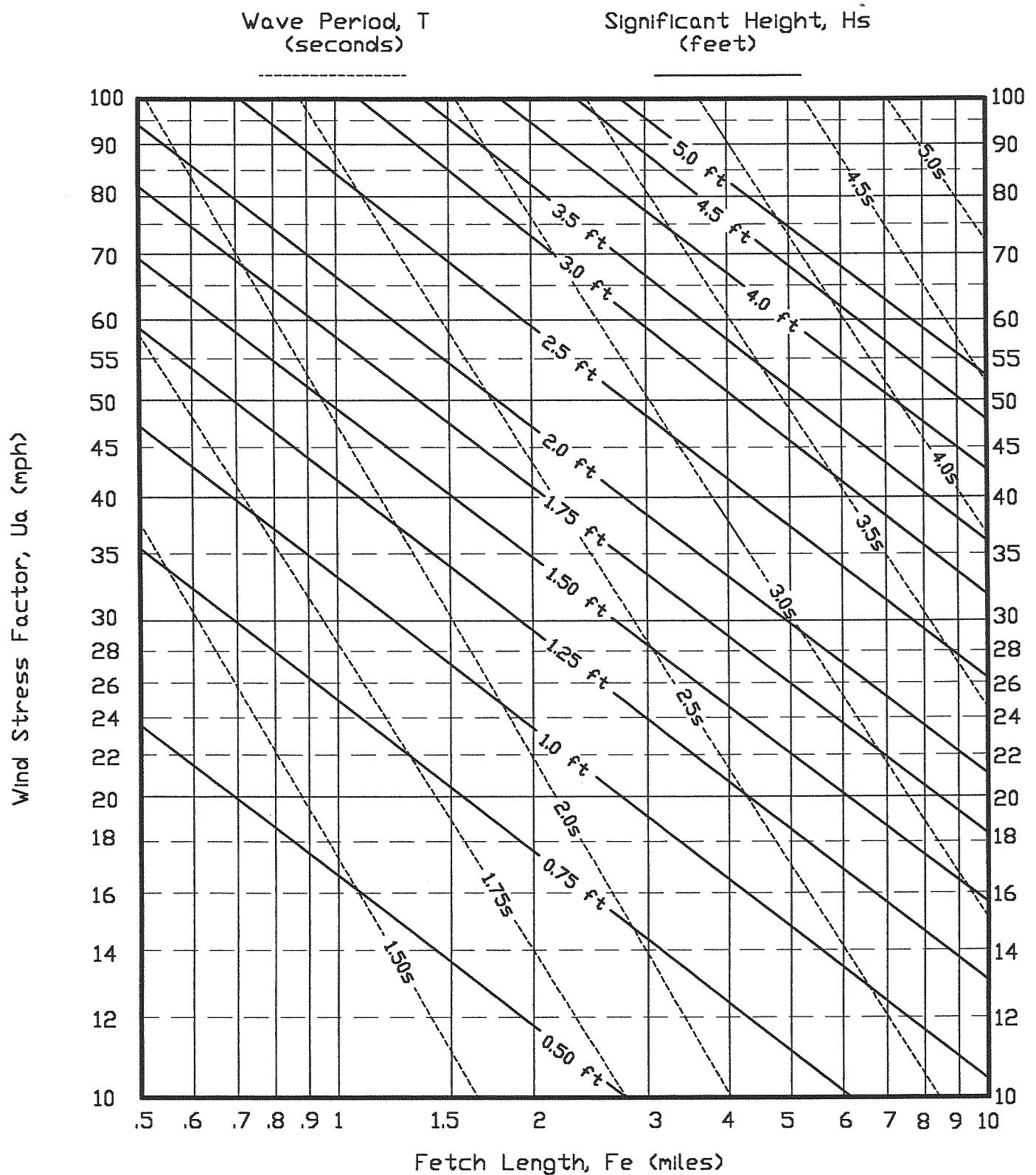
FIGURE 3. Nomograms of deepwater significant wave prediction curves as functions of wind speed and fetch length.
